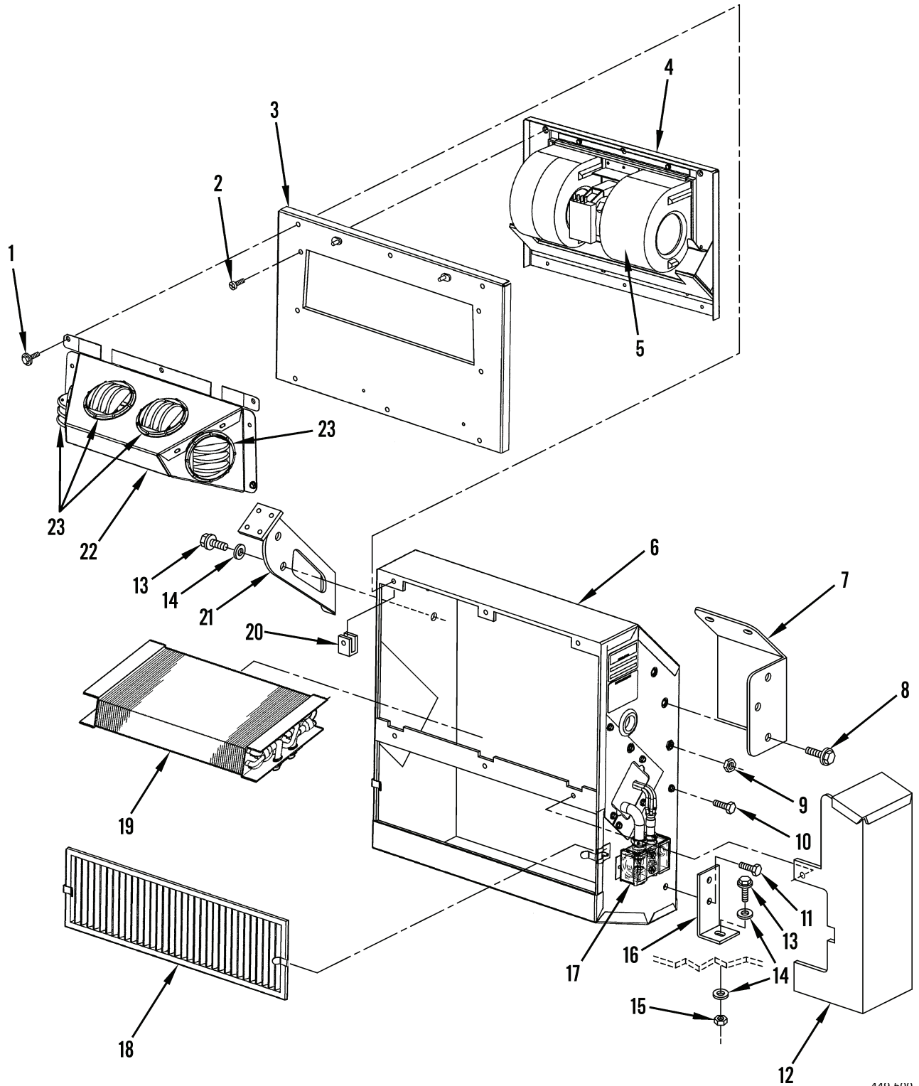
Figure 1. A/C Evaporator Assembly and Mounting Hardware (Sheet 1 of 2)
